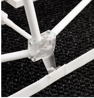
SKU: RPL-BL-HUB-O Outer frame hubs for velcro strips
